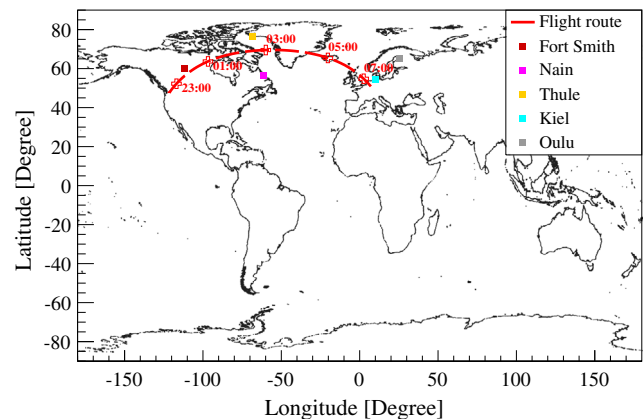
Fig. 1. Flight route from Seattle to Cologne (red dashed line; position of aircraft at different times UTC is indicated by the crosses) and the location of different neutron monitor stations close to the route (coloured squares).
