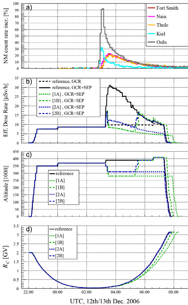
Fig. 2. From top to bottom: (a) relative count rate increases of selected neutron monitor stations located in proximity of the analysed flight route (cf. Fig. 1); (b) calculated effective dose rates from galactic cosmic rays (GCR) and solar energetic particles (SEP) for the different scenarios; (c) altitude profiles of the different flight scenarios; (d) effective cut-off rigidities R_c of the different scenarios.
