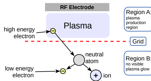
Figure 1: Plasma is generated between an rf electrode and a grid (Region A). Fast electrons pass through the grid and ionize neutral gas atoms on the other side, generating a low temperature electron population (Region B).
