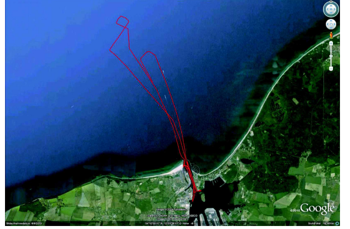
Fig. 3: Route of the ship visualized by the red lines when the receiver was located on the light house.
