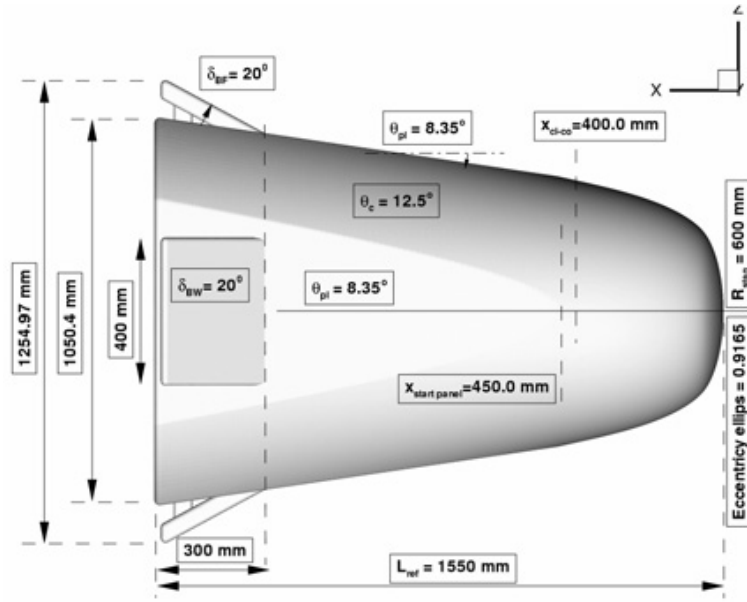
Figure 1: EXPERT 4.4 geometry, real size (from [2])
