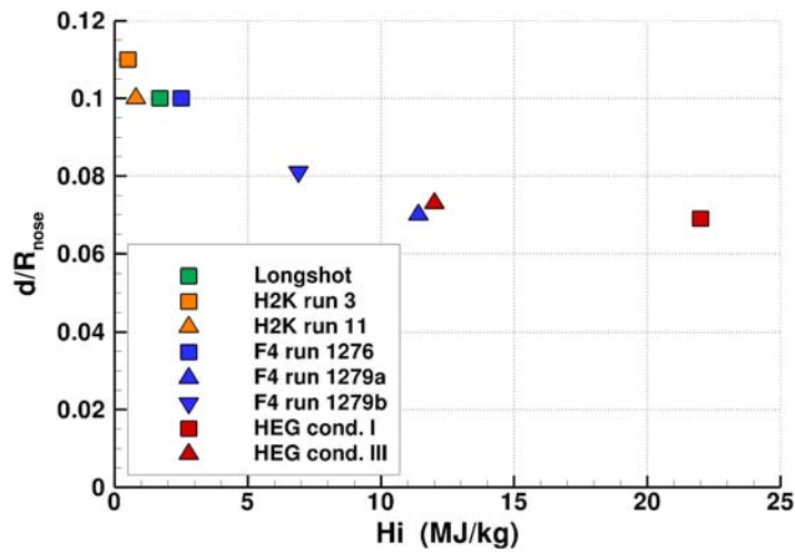
Figure 8: non-dimensional shock stand-off distance along the model x-axis at 5 degrees angle of attack
