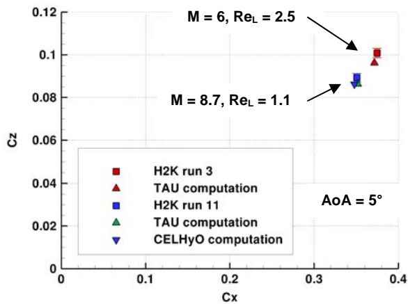
Figure 11: C_x - C_z summary plot for H2K
