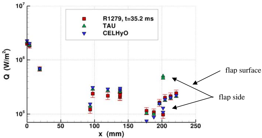
Figure 14: measured and computed wall heat flux, F4 run 1279, t = 35.2 ms
