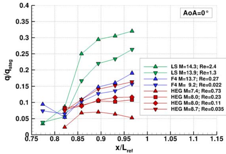
Figure 7: heat flux measurements on the flaps at 0 degree angle of attack
