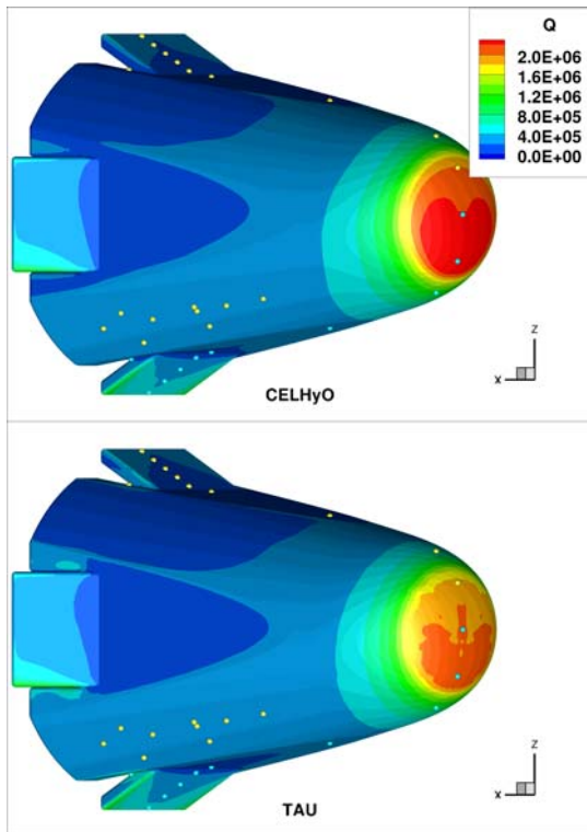
Figure 9: F4 run 1279, t = 35.2 ms, AoA = 5 degrees, wall heat flux and probes positions ; pressure taps (light blue) and thermocouples (yellow)
