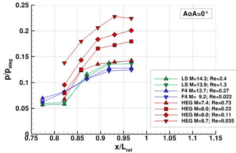
Figure 6: pressure measurements on the flaps at 0 degree angle of attack
