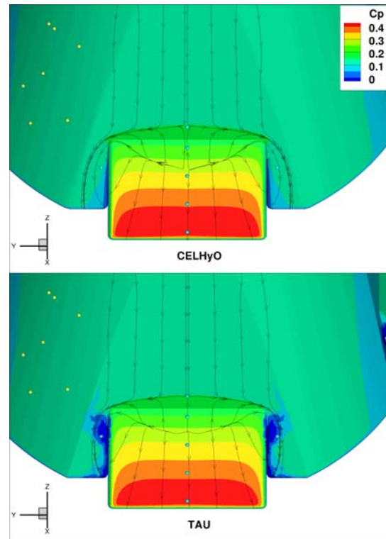
Figure 10: F4 run 1279, t = 35.2 ms, AoA = 5 degrees, wall pressure coefficient and friction lines on the windward flap
