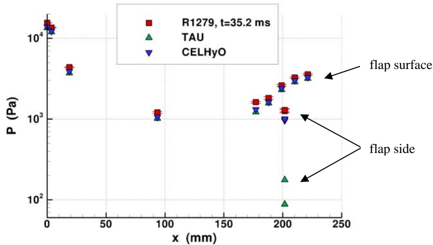
Figure 13: measured and computed wall pressure, F4 run 1279, t = 35.2 ms
