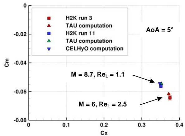
Figure 12: C_x - C_m summary plot for H2K
