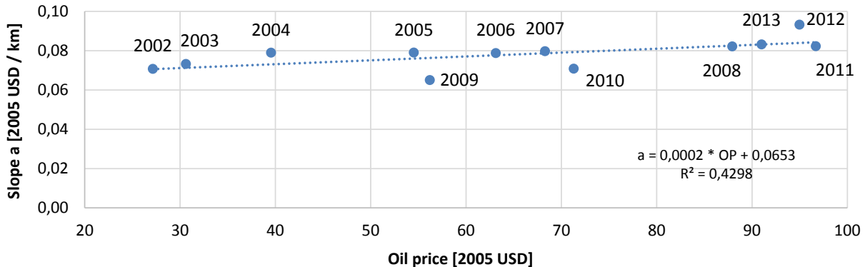
Figure 11: Correlation of the external scenario factor "oil price" and airfare slope a
