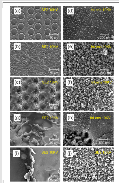
Fig. 6: Pretreatment with 33%, 66% or 100% power, 40KHz, 1x repetition: (a)-(f). (g)-(h) macro and micro structure of a fracture surface covered with PEEK. (i) PEEK rim of at adhesion defect. (j) lasered surface after corrosion.
