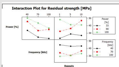
Fig. 5: Interaction between the laser parameters.
