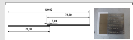
Fig.3: Lap-shear specimen, and photo of laser treated metal stripes.
