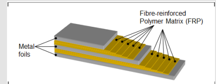
Fig.1: Schematic lay-up of a hybrid material based on adhesive bonding: a laminate with fiber-reinforced polymer matrix, e.g. Titanium/CF-PEEK.
