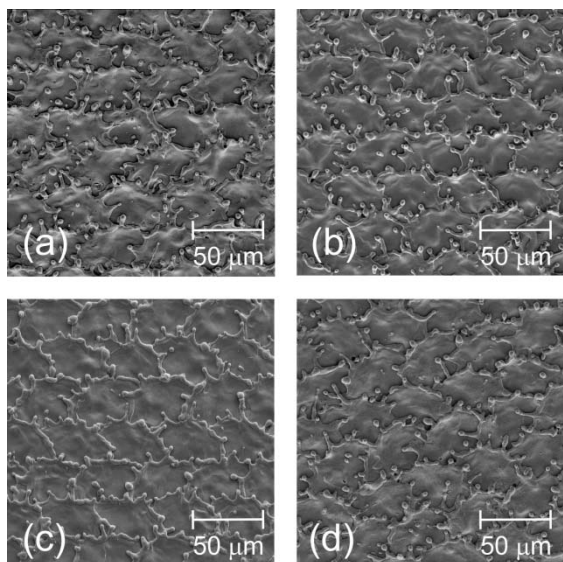
Fig. 5 SEM images (SE2, 10kV) of a \text{TiAl3V2.5} titanium surfaces laser irradiated in (a) air, (b) \text{O}_2 , (c) \text{N}_2 , and (d) Argon. The laser-induced macro-structuring at the micron scale is a clearly distinguishable feature.
