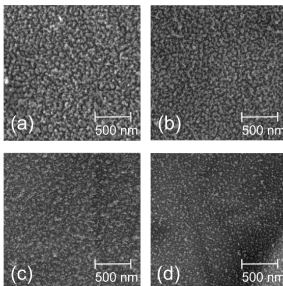
Fig. 6 SEM images (SE2, 10kV) of a \text{TiAl3V2.5} titanium surfaces laser irradiated in (a) air, (b) \text{O}_2 , (c) \text{N}_2 , and (d) Argon showing the laser-induced nanostructuring of the functional adhesive interface.
