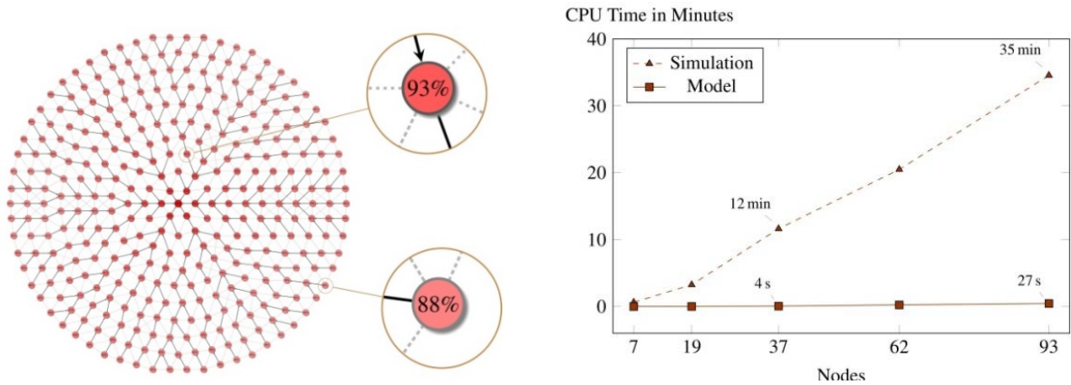
Fig. 3. Left: Depiction of the analytical mode results for a subnetwork of 340 nodes and 10 s packet interval. Right: Comparison of required time for computation for simulation and analytical model.
