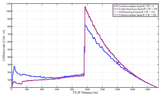
Fig. 7. Total collision rate over the distance between the two colliding transmitters for all considered approaches (distance resolution = 10 m).
