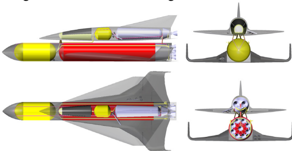
Figure 1. General configuration architecture of the SpaceLiner configuration 7-2
