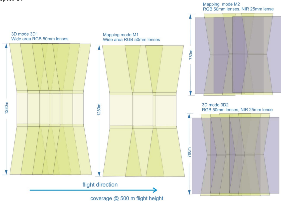
Fig. 5: Footprints of different 3D and mapping mode configurations
