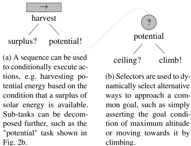
Figure 2: In a behavior tree, simple tasks are connected to a tree in order to achieve more complex goals.
