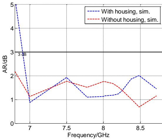
Figure 8. Simulated axial ratio of the antenna array
