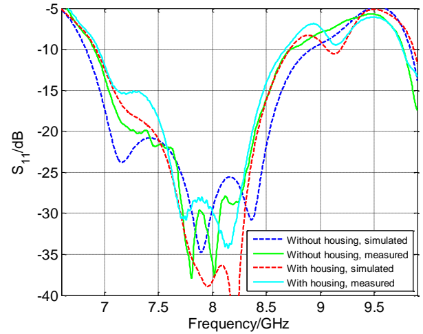
Figure 6. Input reflection coefficient S_{11} of the 2 \times 2 array
