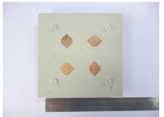
Figure 3. Top view of milled patch array, only the upper layer is visible
