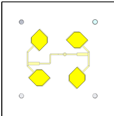
Figure 2. Schematic top view of patch array. The structure on the lower layer is shown in light yellow
