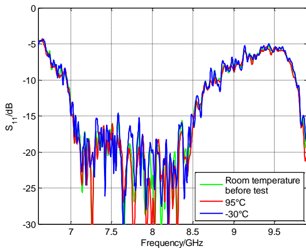
Figure 9. Input reflection coefficient S_{11} of the antenna array under different temperature conditions
