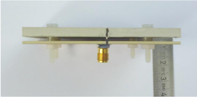
Figure 4. Side view of milled patch array
