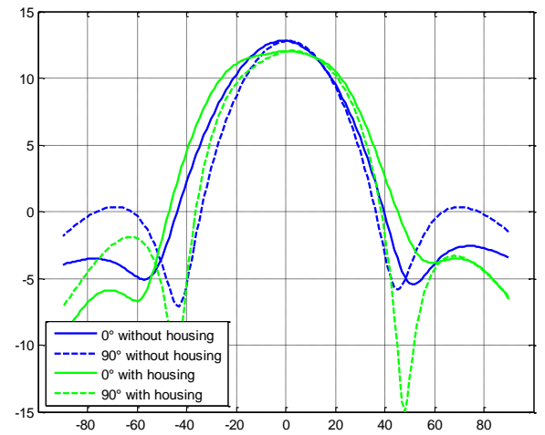
Figure 7. Simulated radiation pattern for 8.25 GHz
