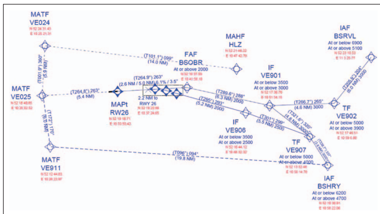
Figure 3. RNAV and RNP procedures for Brunswick (EDVE) in detail.
