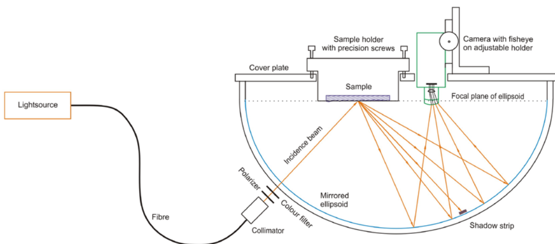
Figure 2: Scheme of instrument
