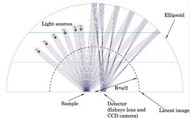
Figure 1: Raytracing model of beam paths
