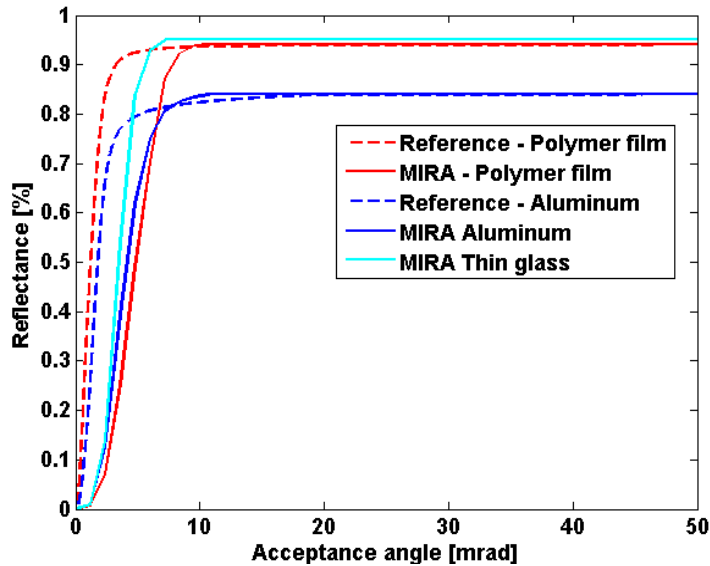
Figure 7: Comparison of the measurement data from MIRA with data generated with the goniometer from pab , circular acceptance aperture, 15° incidence angle, wavelength 650 nm
