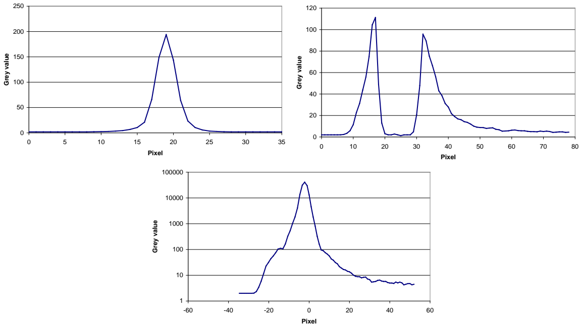
Figure 5a: Intensity distribution along a line crossing the peak; b) Intensity distribution along a line crossing the peak with shadow strip in the up-down direction on Figure 4b (the left part of the distribution is influenced by the opening in the ellipsoid for the incident light); c) Stitched intensity distribution of a) and b) after conversion of the peak measurement to match the integration time of the shadow strip measurement.
