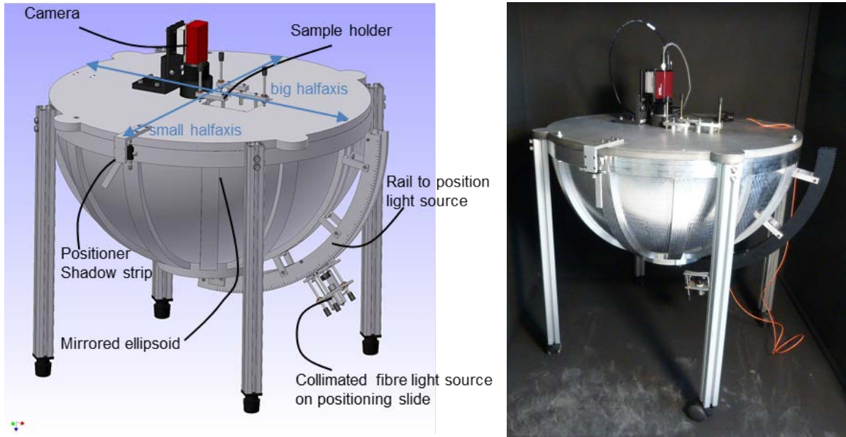
Figure 3: Construction sketch of instrument and mounted prototype
