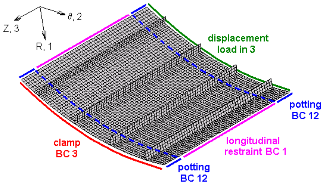
Figure 5: D2 FE model with boundary condition (BC) definition.
