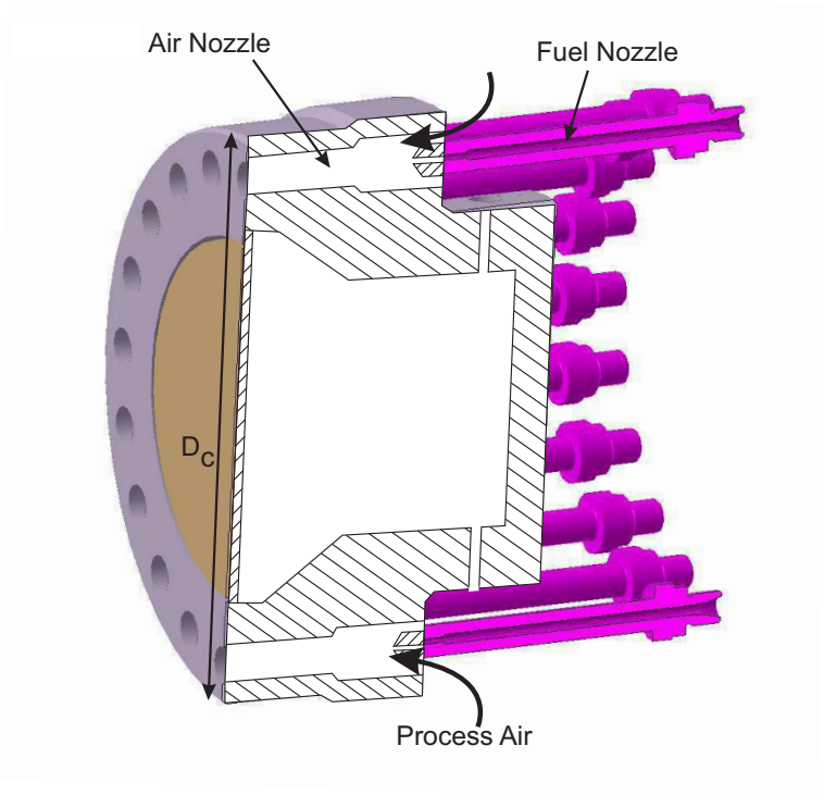
Figure 1. Uncooled Combustor.
