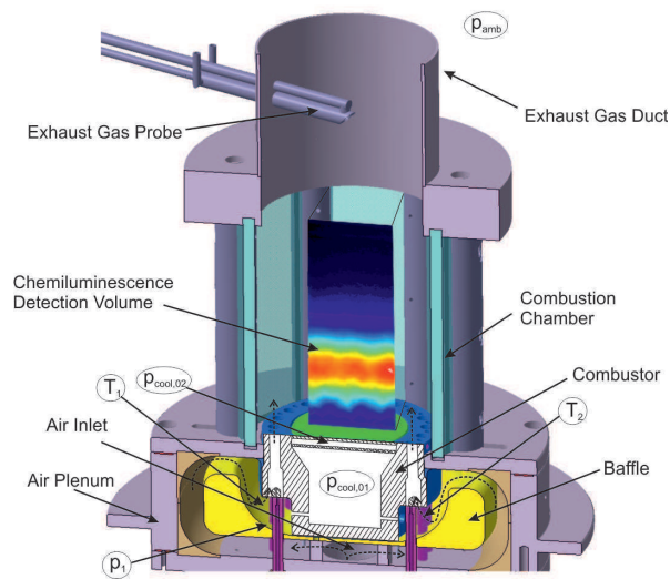
Figure 3. Atmospheric Combustor Test Rig
