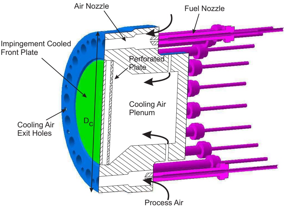
Figure 2. Impingement Cooled Combustor.
