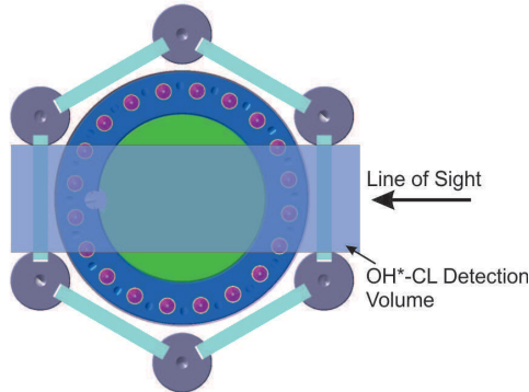
Figure 4. Line of Sight of the OH*-CL measurements
