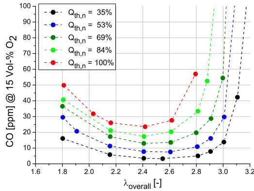
Figure 7. CO Emissions of the Uncooled Combustor Configuration.
