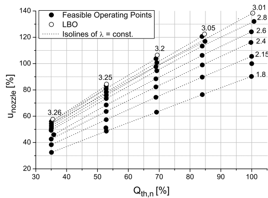
Figure 5. Operating Range of Uncooled Combustor Configuration.
