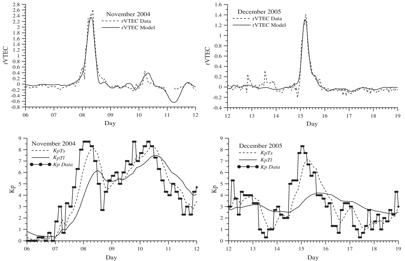
Fig. 14. (Upper row of plots) Comparison between the observed (dashed line) and model (solid line) rVTEC at the geographic point ( 20^\circ N, 130^\circ W) for the geomagnetic storm in November 2004 (left plot) and December 2005 (right plot); (bottom row of plots) Comparison between the measured Kp-index (tick solid line with dots) and modified Kp TS – (dashed line) and Kp TI – (solid line) indices for November 2004 (left plot) and December 2005 (right plot) (Andonov et al. 2011).
