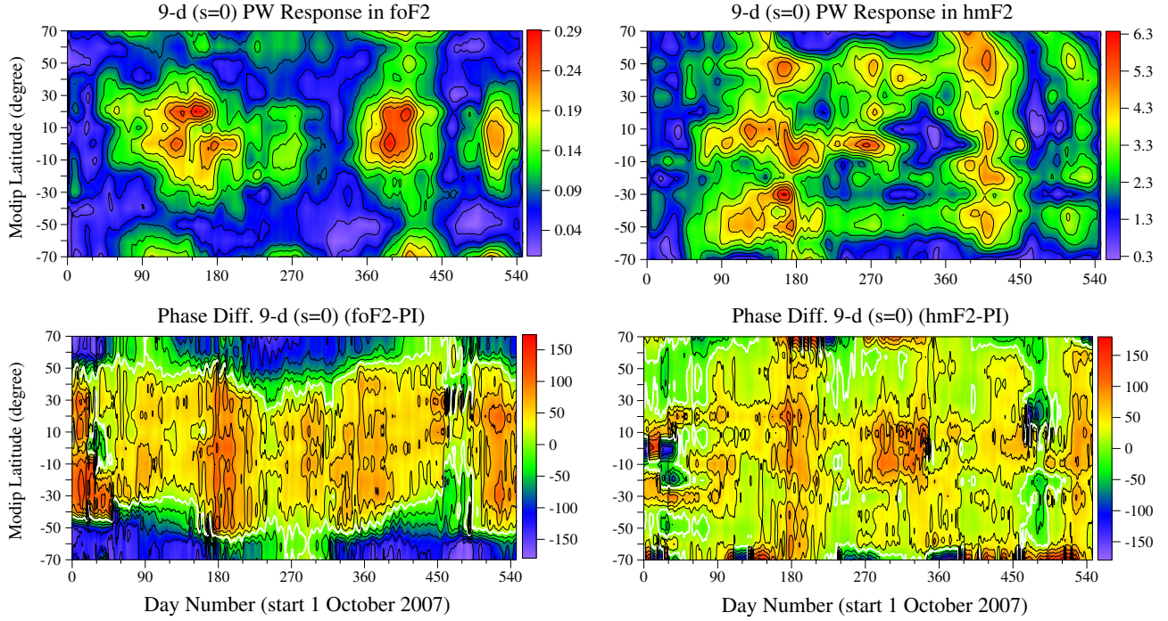
Fig. 3. (Upper row of plots) Extracted from the COSMIC data 9-day zonally symmetric ( s = 0 ) waves seen in the ionospheric parameters: foF2 (left plot) and hmF2 (right plot); (bottom row of plots) Phase difference between the ionospheric parameters foF2 and the PI (left plot) and between hmF2 and PI (right plot); the thick white line shows the zero phase difference (Mukhtarov & Pancheva 2012).
