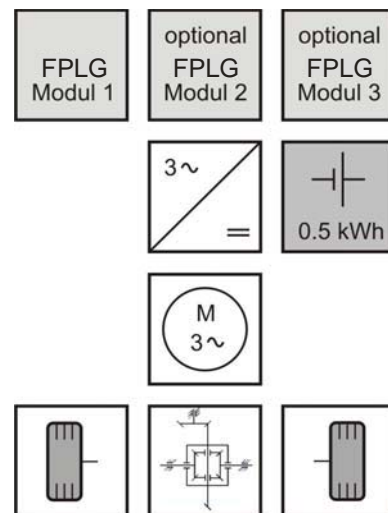
Figure 2: FPLG integrated in a hybrid vehicle
