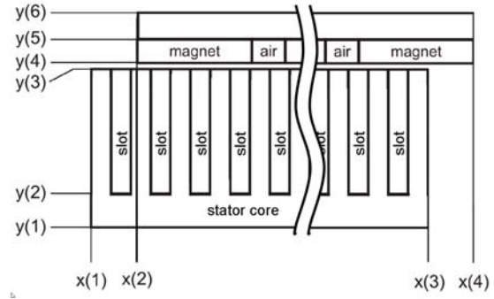
Figure 6: 2-D FEA Model
