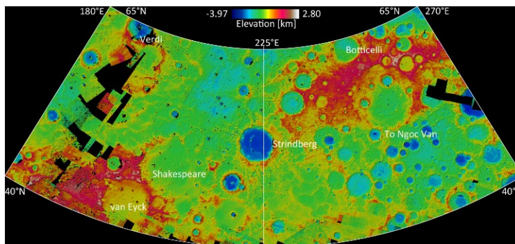
Fig. 3. Strindberg DTM (hill-shaded color-coded heights) with a lateral spacing of 330 m in Lambert two-parallel (conformal) projection. Black areas are gaps in the current stereo coverage. Updated versions of this model will be available at the time of the conference.
