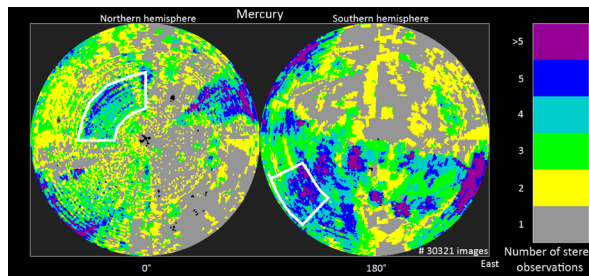
Fig. 1. Stereo coverage of MDIS images having spatial resolutions better than 500 m/pixel. Colors indicate the number of stereo observations that meet the conditions from Table 1 (status as of December 2011). The white polygons mark areas for which sample stereo analysis is reported here.
