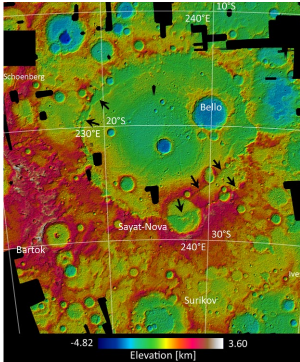
Fig. 2. Beethoven DTM (hill-shaded color-coded heights) with a lateral spacing of 330 m in stereographic (conformal) projection centered at Beethoven basin (20°S, 236°E). Black areas are gaps in the current stereo coverage. Updated versions of this model will be available at the time of the conference.
