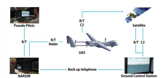
Figure 3 Functional set-up
