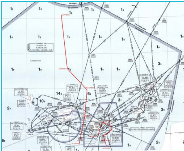
Figure 4 Design of emergency routes
