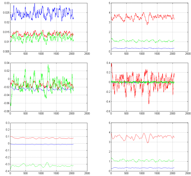
Figure 9. Simulation at 5m Distance, Top: Filter Error, Middle: Controller Performance, Bottom: Total Performance, Left: Position [m] (blue: x, red: y, green: z), Right: Attitude [deg] (blue: roll, red: pitch, green: yaw), abscissa: time [s]
