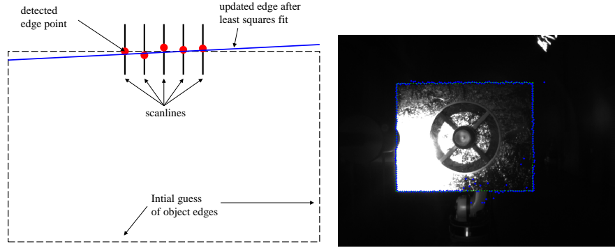
Figure 1. Illustration (left) and results (right) of the edge tracking algorithm
