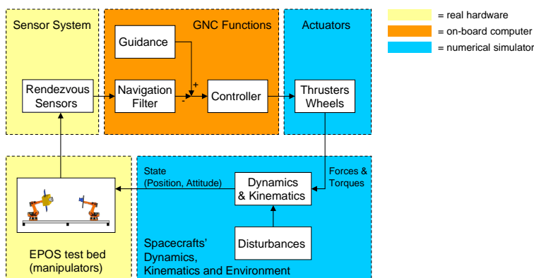
Figure 7. Rendezvous control loop
