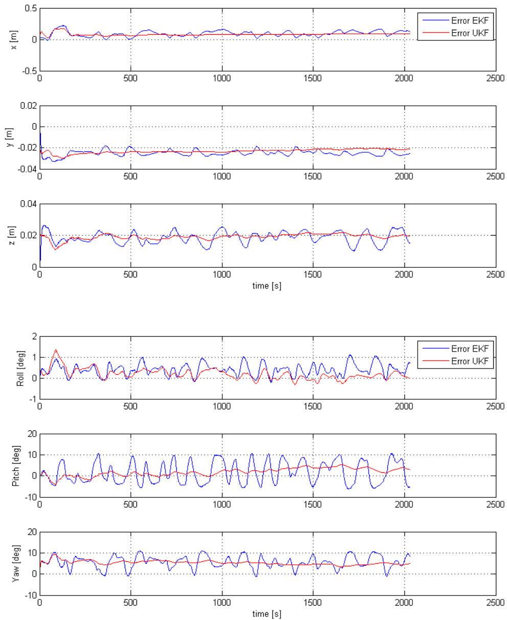
Figure 8. Simulation at 20m Distance, Top: Position Error of EKF and UKF, Bottom: Attitude Error of EKF and UKF
