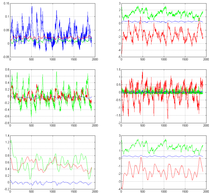
Figure 10. Simulation at 20m Distance, Top: Filter Error, Middle: Controller Performance, Bottom: Total Performance, Left: Position [m] (blue: x, red: y, green: z), Right: Attitude [deg] (blue: roll, red: pitch, green: yaw), abscissa: time [s]
