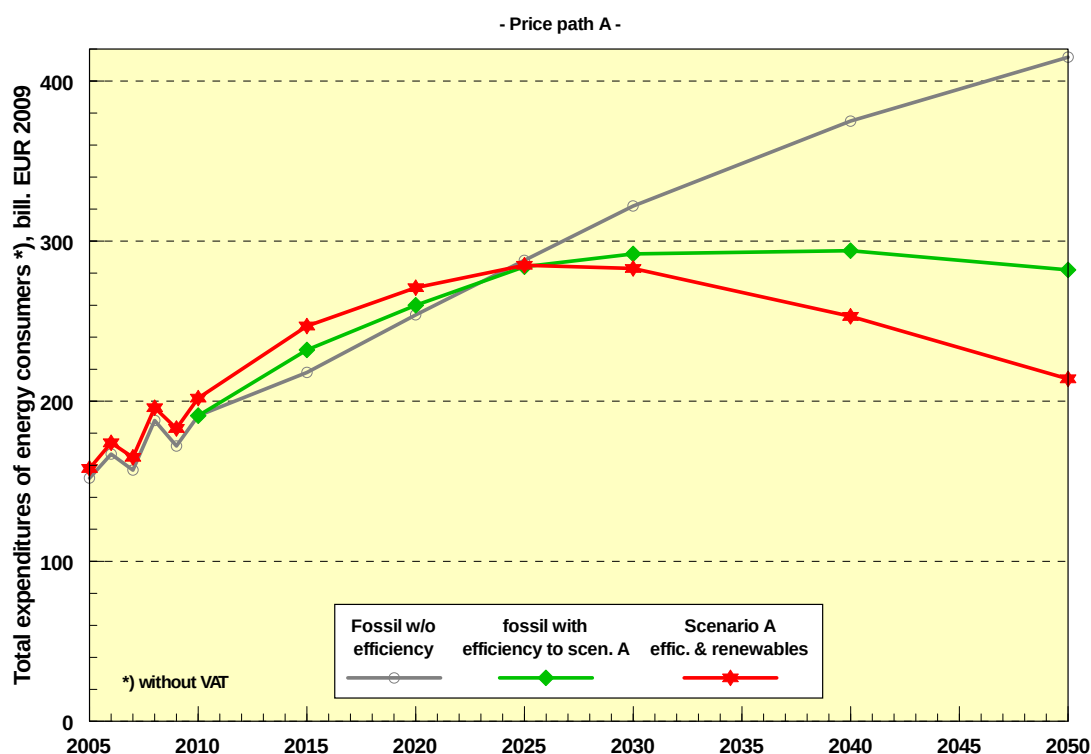
Figure 21: Total expenditures on energy of all consumers for provision of the present consumption level entirely from fossil fuels, if the efficiency goals are implemented, and for the energy mix of Scenario 2011 A
