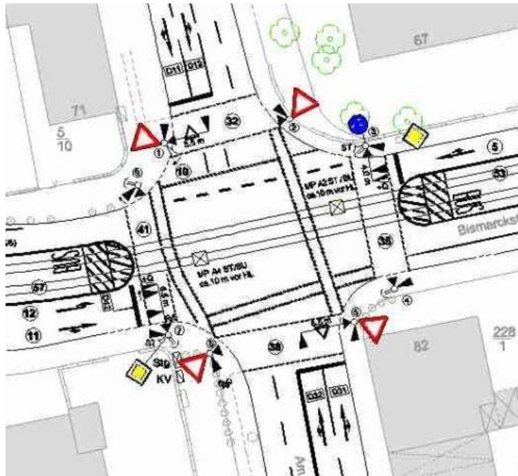
FIGURE 2 Intersection layout.
