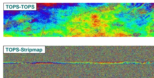
Figure 8. Interferometric phase of one TOPS burst generated by the combination of two TOPS images (up) and a TOPS and a stripmap image (down).
