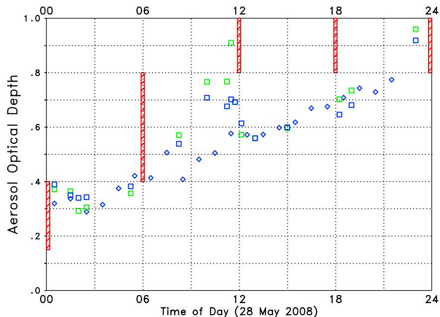
Figure 10. Aerosol optical depth from ground to 4 km derived from integrating lidar measurements of \alpha_p : 355 nm in blue, 532 nm in green, diamonds of POLIS, squares for MULIS. The corresponding DREAM forecasts (36 hours to 60 hours) of \tau_p -ranges at 550 nm are plotted in red: 0.15–0.4, 0.4–0.8 and 0.8–2.5.
