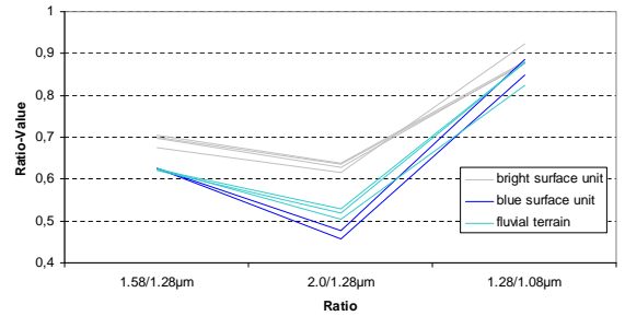
Figure 3: Ratio-spectra of the bright, blue, and fluvial surfaces. Extracted from western Xanadu, VIMS-observations T012.
