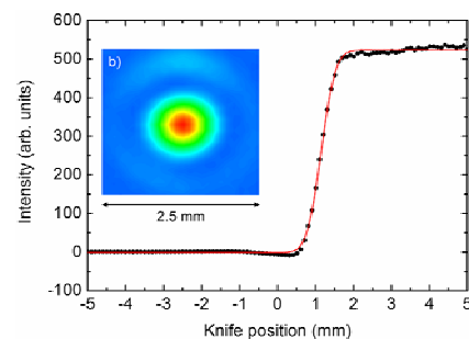
Fig. 1: Beam profile at the position of the minimum waist by scanning a sharp metal blade. The output power is well above 1mW at 3.1 THz.
