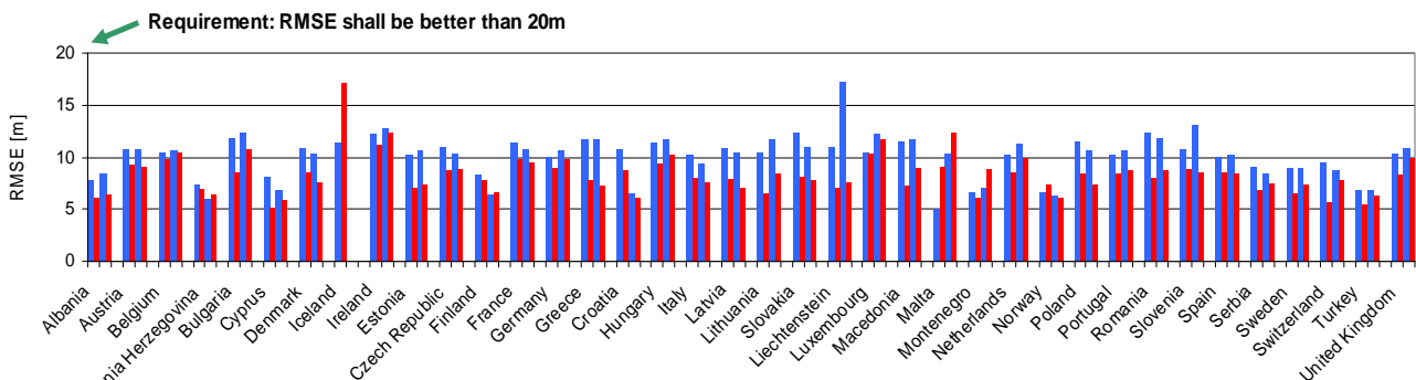
Figure 3 Geometric accuracy (RMSE) of Image2006 products w.r.t. reference images (relative accuracy). RMSE x (blue) and RMSE y (red) for European coverage 1 (first two columns of country) and European coverage 2 (last two columns of country)
