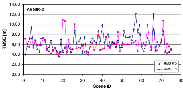
Figure 4 Geometric accuracy (RMSE) of ALOS AVNIR-2 orthorectified scenes w.r.t. reference images (relative accuracy). RMSE x (blue) and RMSE y (red)
