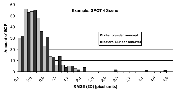
Figure 2 Histogram of the residuals ( RMSE_{xy} ) after least squares adjustment for one SPOT 4 HRVIR scene. Dark bars: before blunder removal; bright bars: after blunder removal using 2 pixel sizes as GCP rejection level.
