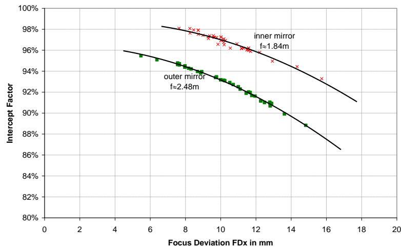
Figure 5: Intercept factor ray-tracing results for EuroTrough (RP3) mirror panels assuming a typical sun-shape and including typical tolerances for the rest of the collector components, for 0° incidence angle
