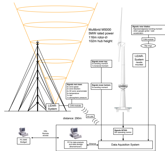
Fig. 3: Overview of the measurement system
