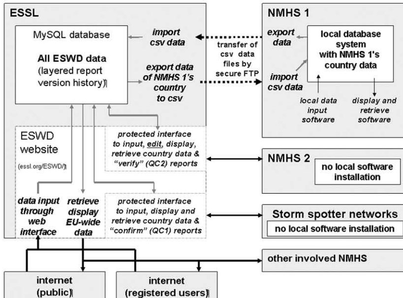
Fig. 2. Schematic of the ESWD data stream between the central ESSL server, local installations at collaborating NMHS, as well as registered users and the public. (a) ESWD version 2 setup with exemplary partners DWD and ZAMG. Note the exchange of files, not parts of a relational database. (b) Situation with the new ESWD version 3, based on a MySQL database on the ESSL server. Here, NMHS have more options to collaborate with the ESWD, e.g., NMHS 1 via true database exchange, NMHS 2 via a customised user portal at ESSL, or in the simplest case via the public ESWD portal.
