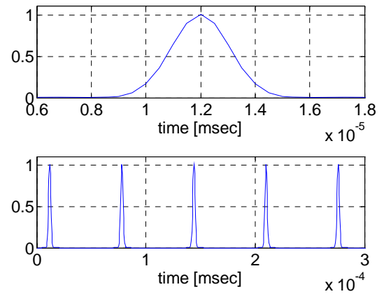
Figure 2: Normalized DME like pulse (time domain)
