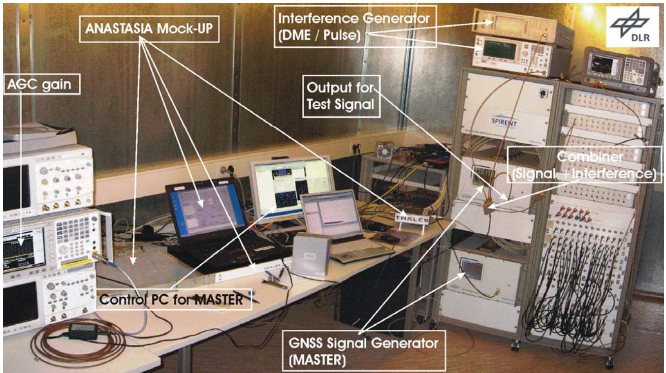
Figure 14: Photo of test setup.
