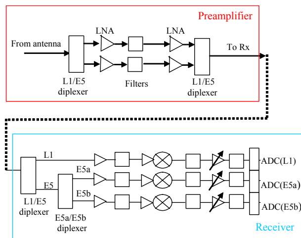
Figure 7: Preamplifier and receiver RF architecture
