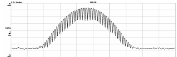
Figure 3: DME like pulse (frequency domain)
