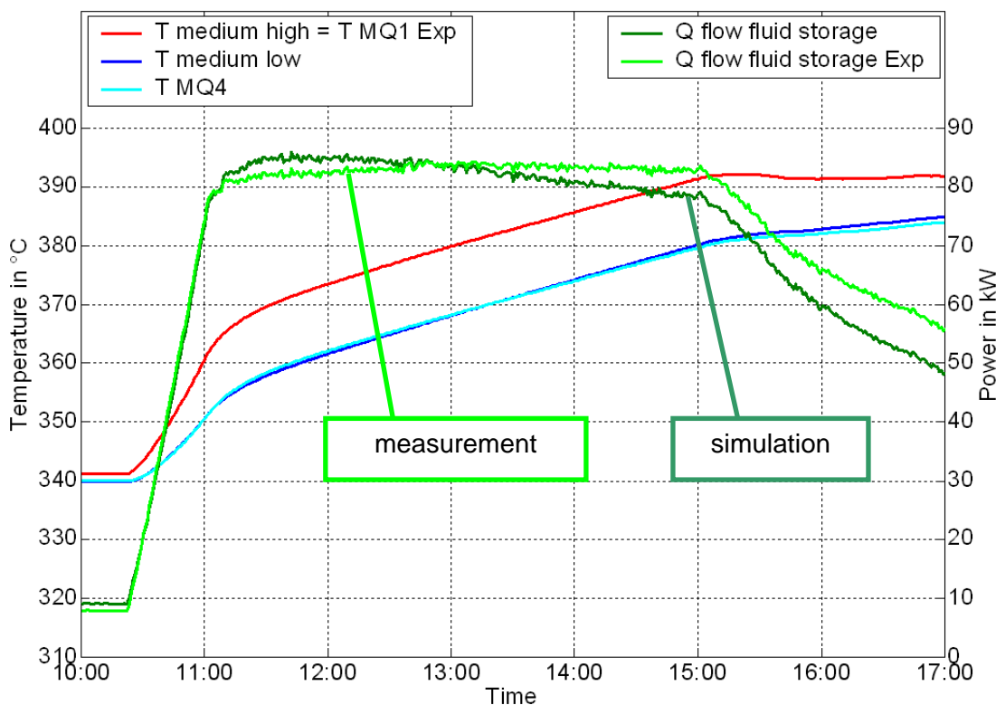
Figure 5: Comparison of simulation and experiment
