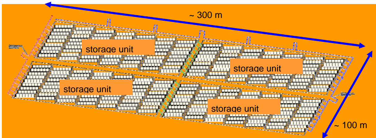
Figure 6: Set-up of a 1100 MWh concrete storage from 252 basic storage modules
