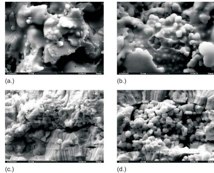
Fig.1. SEM micrographs of conventional and nanostructured as-sprayed YSZ,
