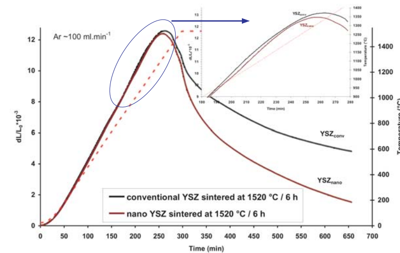
Fig.4. Dilatometer data of YSZ conv / nano layers; heating rate 5 °C.min -1 , holding time 6 h at 1520 °C; Included figure: curve maxima in detail
