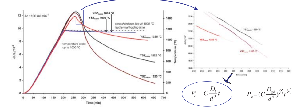
Fig.5. Dilatometer data of free standing YSZ conv / nano samples sintered at 1000 °C, 1325 °C, and 1520 °C; right diagram: detailed curve with trend line; reflecting the intermediate stage of sintering
