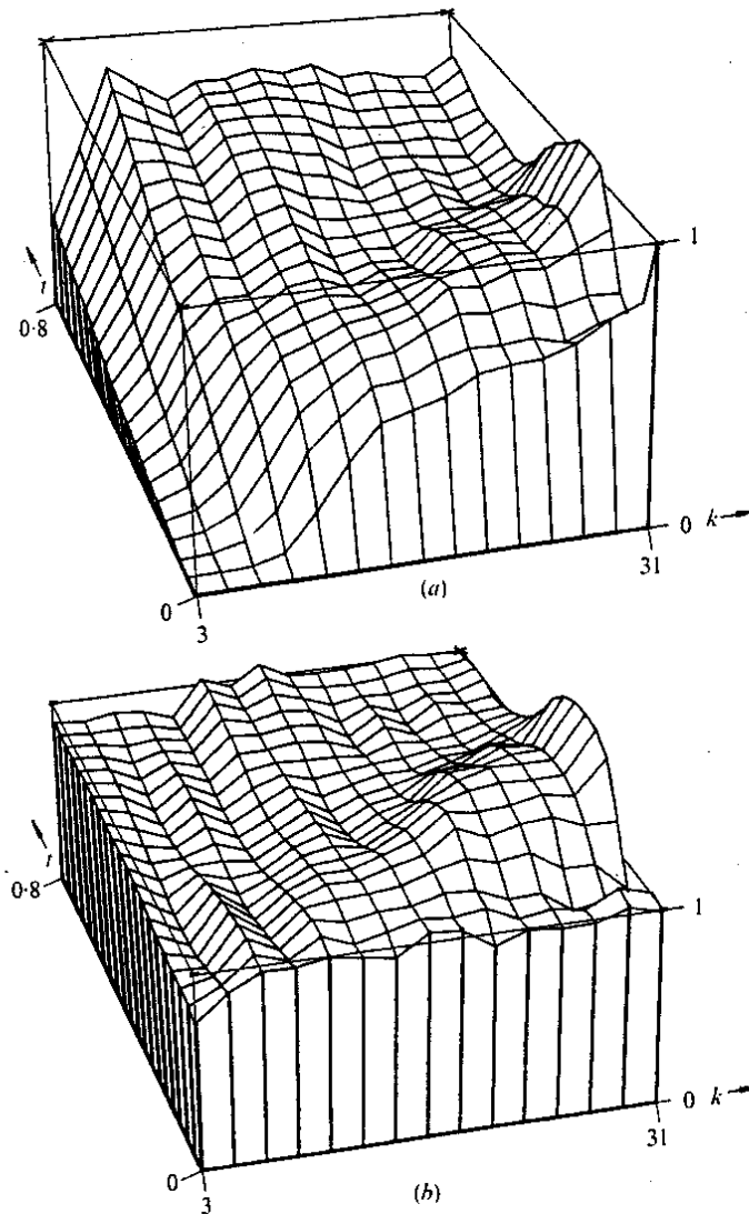
FIGURE 6. Energy ratios vs. wavenumber ( k = K ) and time ( t = T ) for run A1. The crosses denote unity. 3 \leq k \leq 31 , 0 \leq t \leq 0.8 . (a) \hat{E}_{33}/\hat{E}_{11} . (b) \hat{E}_{23}/\hat{E}_{11} .
