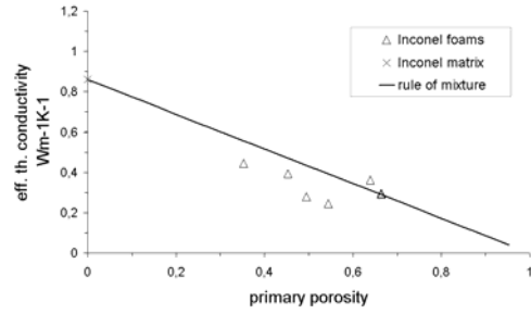
Figure 2: Effective thermal conductivity of selected Inconel foams as a function of their total porosity
