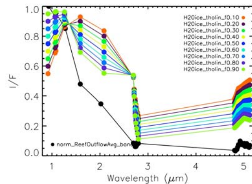
Fig. 4: Preliminary checkerboard model of two-component mixtures of Titan tholin and water ice, as compared to normalized VIMS surface signatures from T20. “fX.XX” indicates the percentage of water ice in each mixture (i.e., “f0.10” is 10% water ice, 90% tholin). Water ice is a better match than tholin to the gross behavior of the average terrain.
