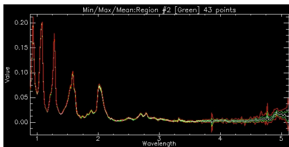
Fig. 2: Calibrated I/F as a function of wavelength for the average terrain in Fig. 1 (“ReefOutflowAvg” in Figs. 3, 4). The spectrum displays peaks not seen in other Titan surface spectra prior to T20.
