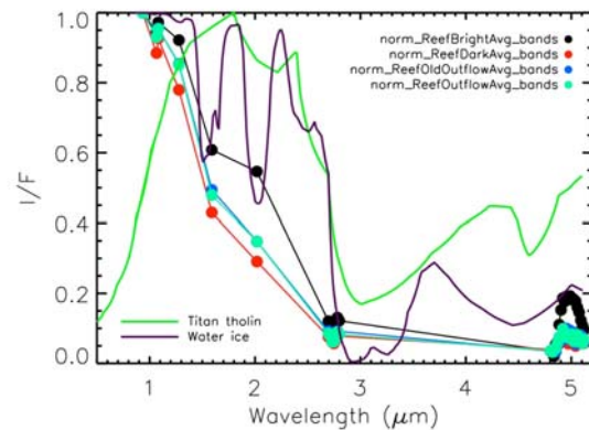
Fig. 3: For the T20 VIMS spectra, the mean I/F from terrain in each colored region of Fig. 1 was first normalized, then wavelength bands at the methane windows were isolated (colored dots) to characterize the gross spectral behavior of the terrains. Laboratory reflectance spectra of Titan tholin (green line) and water ice (purple line) were regridded to VIMS wavelength bins via cubic spline interpolation.
