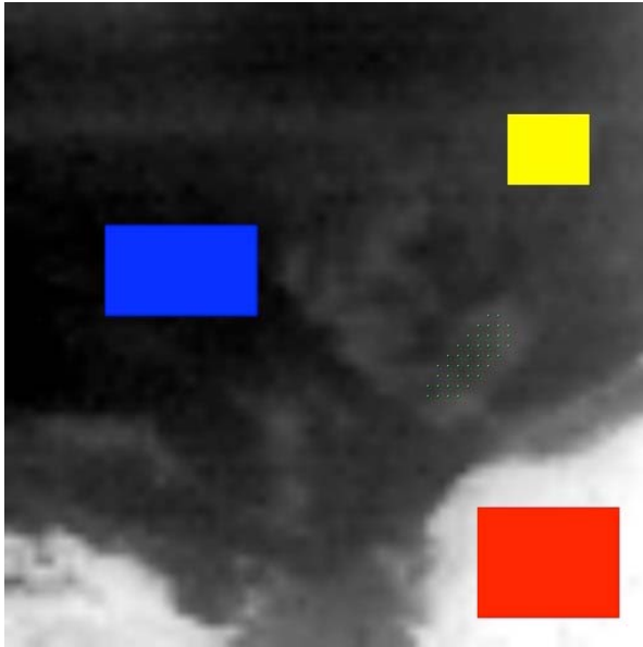
Fig. 1: A 64 x 64 pixel VIMS image of Bohai Sinus (“Pacman Bay”), acquired during Cassini’s T20 Titan flyby (sequence 031TI, observation COMPMAP101, VIMS prime, 80 ms integration time). The phase angle was 12 degrees; spacecraft range was 3886 km. Color differences are seen between bright and dark albedo terrains within Bohai Sinus; colored boxes indicate areas for which VIMS spectra were extracted for further analysis.
