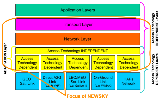
Figure 3. Potential NEWSKY protocol design.
