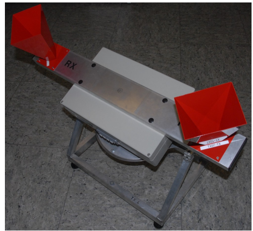
Fig. 6. Active target (transponder). The transponder housing including the antennas can be rotated which results in different scattering matrices.
