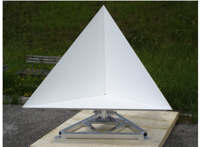
Fig. 2. Passive calibration target: Trihedral corner reflector with an inner leg length of 1.5 m.
