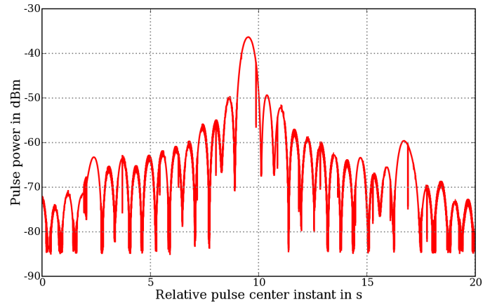
Fig. 5. Recorded datatake from a ground receiver showing the azimuth pattern.
