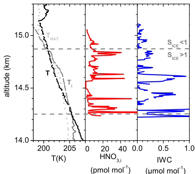
Fig. 4. Vertical profiles of T , T_{NAT} , T_i , particle HNO_3 and IWC during ascent through the cirrus cloud.
