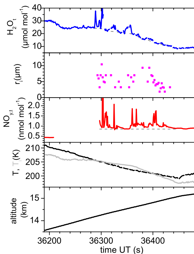
Fig. 3. Time series of total H_2O_t , mean particle radii, total NO_{y,t} , T , T_i and altitude measured on 17 February 2005 during ascent from Araçatuba (19.7° S, 50.2° W, Brazil). Spikes in the NO_y and H_2O signals indicate the presence of HNO_{3,i} in ice crystals. NO_{y,t} and H_2O_t data are not corrected for particle enhancement. The gray lines are estimates for NO_{y,r} and H_2O_r in the particle layer.
