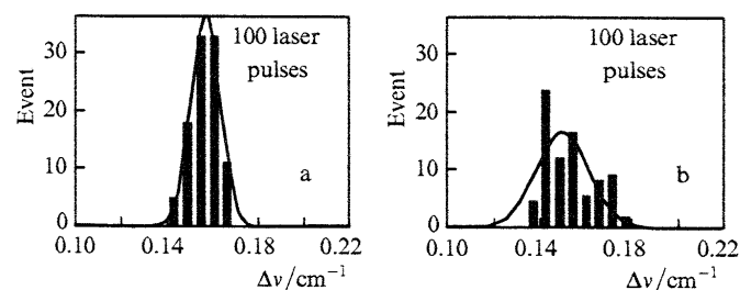
Figure 4. Histograms of the Q_1 linewidths in hydrogen measured by the DBB-CARS (a) and BB-CARS methods under identical experimental conditions in the H_2-N_2 mixture (the H_2 and N_2 pressure is 1 and 40 bar, respectively) at room temperature. The average linewidth is 0.16\text{ cm}^{-1} , the histogram width for the DBB-CARS and BB-CARS configurations is 0.006 and 0.017\text{ cm}^{-1} , respectively.
