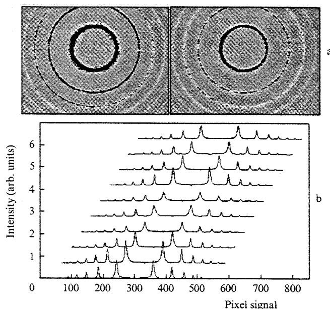
Figure 3. (a) Circular structure of Fabry-Perot interferograms for two successive laser pulses (DBB-CARS configuration) obtained in a cell with the H_2-N_2 mixture (the H_2 and N_2 pressure is 3 and 14 bar, respectively) at room temperature (only random speckle-modulation of the circular pattern is observed over the entire light field) and (b) the results of angular integration of interferograms for a series of 10 laser pulses obtained in the DBB-CARS configuration in a cell with the H_2-N_2 mixture (3 and 14 bar, respectively) at room temperature; all the spectral lines have good quality and are suitable for further processing.
