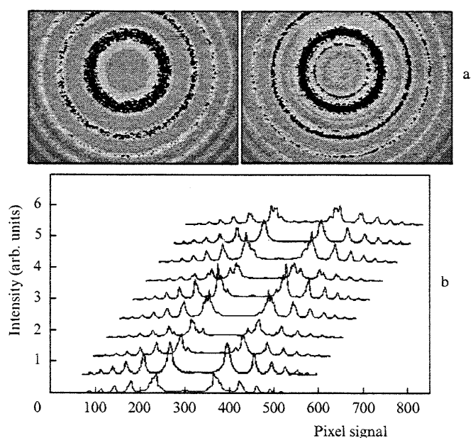
Figure 2. (a) Circular structure of Fabry-Perot interferograms for two successive laser pulses (BB-CARS configuration) obtained in a cell with the H_2-N_2 mixture (the H_2 and N_2 pressure is 3 and 42 bar, respectively) at room temperature (random speckle-modulation of the circular pattern is observed over the entire light field, as well as the fluctuating substructure of interference fringes caused by the spectral fluctuations of a Stokes laser from pulse to pulse) and (b) the results of angular integration of interferograms for a series of 10 laser pulses obtained in the BB-CARS configuration in a cell with a H_2-N_2 mixture (3 and 42 bar, respectively) at room temperature; the random intensity modulation of spectral lines caused by fluctuations of the spectrum of the Stokes laser from pulse to pulse are clearly observed; the further processing of the spectra requires selection.
