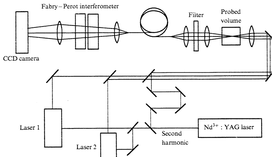
Figure 1. Optical scheme of the experimental setup.
