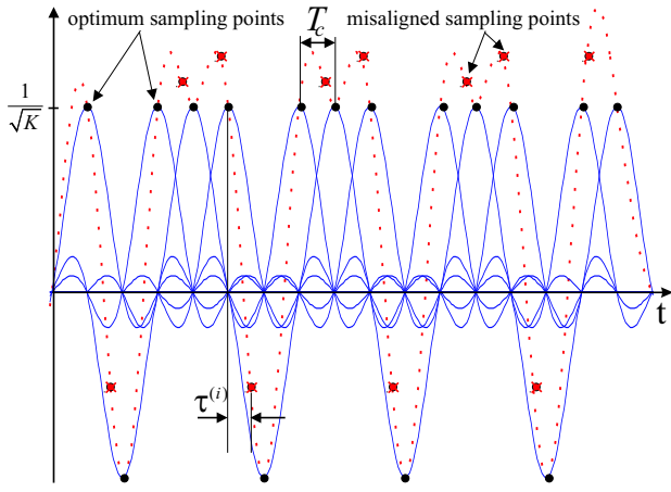
Fig. 2. Example of the IFDMA signal after the receive filter. Sampling time offset \tau^{(i)} causes SNR degradation and leads to ISI; \mathbf{d}^{(i)} = [1, -1, 1, 1]^T ; L = Q = 4 ; \alpha = 0.25 ; only user i = 0 is active; AWGN channel with a negligible noise power.
