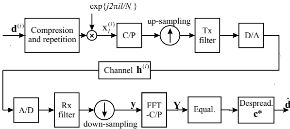
Fig. 1. Simulation model for IFDMA uplink
