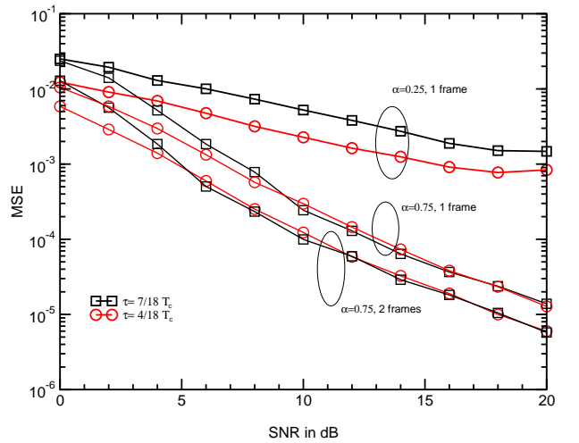
Fig. 4. MSE of the sampling time offset estimate versus SNR
