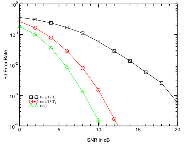
Fig. 3. BER versus SNR for the different values of sampling time offset \tau ; \alpha = 0.25
