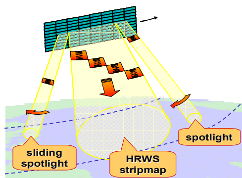
Figure 7. Hybrid SAR imaging modes.
