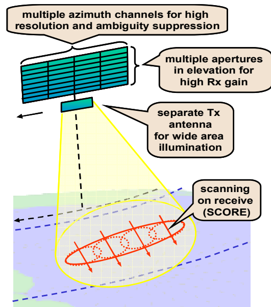
Figure 1. High-Resolution Wide-Swath (HRWS) SAR System.
