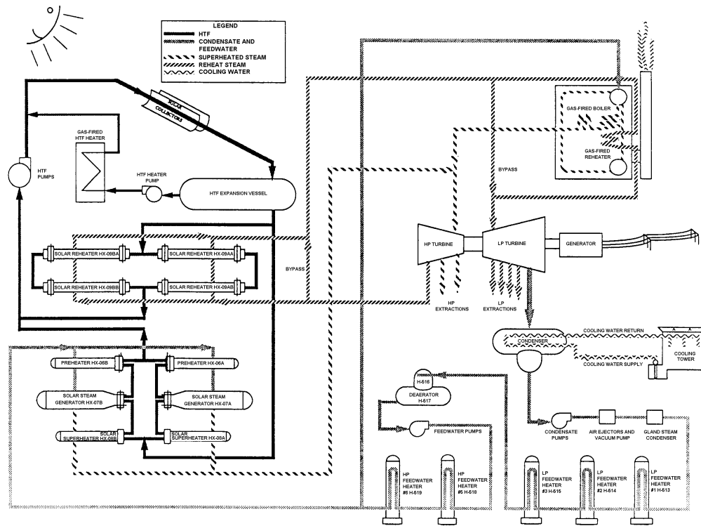
Fig.2. Schematic of the SEGS VI plant.
