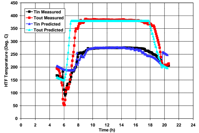
Fig. 6. Measured and predicted HTF temperatures at the inlet and outlet of the trough field on 7/18/91.
