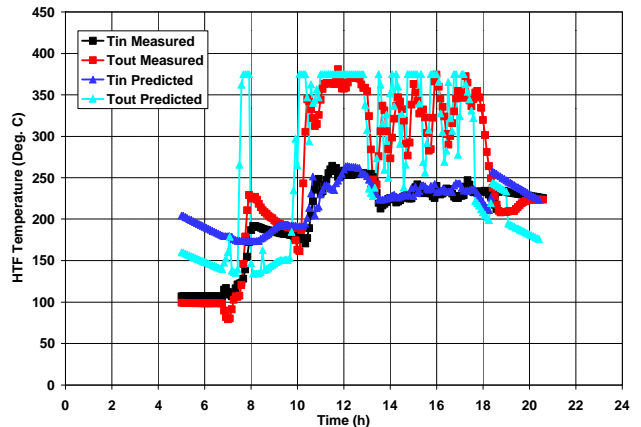
Fig. 7. Measured and predicted HTF temperatures at the inlet and outlet of the trough field on 9/19/91.
