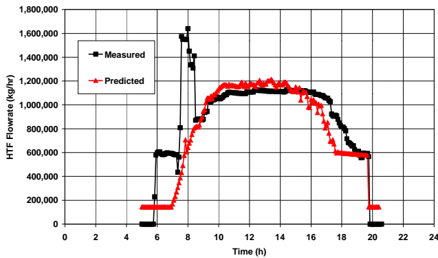
Figure 8. Measured and predicted HTF flow rate on 7/18/91.
