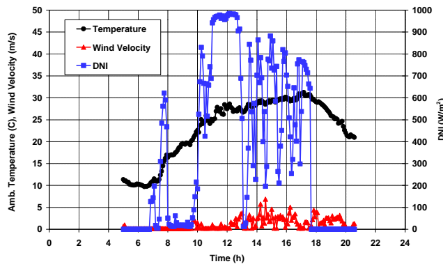
Fig. 5. Weather conditions on 9/19/91.
