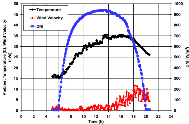
Fig. 4. Weather conditions on 7/18/91.
