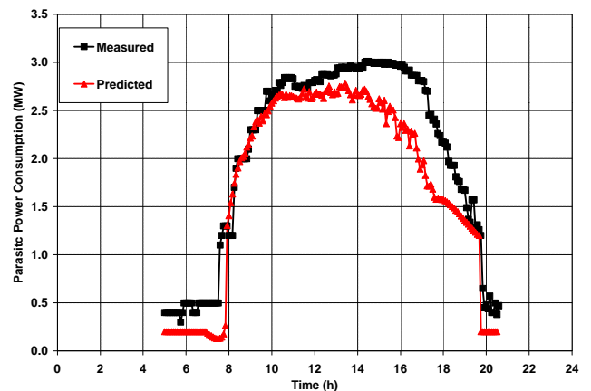
Figure 16. Measured and predicted parasitic power use on 7/18/91.
