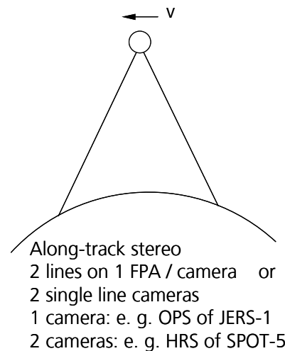
Figure 4 Along-track stereo with 2 sensors
