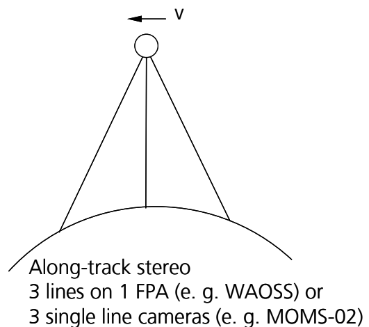
Figure 5 Along-track stereo with 3 sensors
