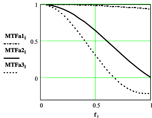
Figure 8 Influence of a_{LM} on MTF_{LM} with a_{LM} = 0.1, 1, 1.5 \cdot \text{GSD}
