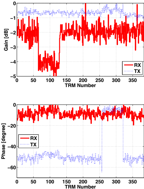
Fig. 5. Module level measurements of antenna in TX and RX. Each data set is referenced to its maximum value. Above - Gain degradation of -2.4 dB in RX for TRMs 64 to 127 corresponding to panels 2 and 3. Below - Phase degradation of +45^\circ at TRMs 256 to 319 corresponding to panels 8 and 9.
