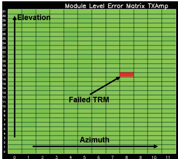
Fig. 3. Error Matrix of TerraSAR-X antenna. TX gain estimation derived from module level check with one TRM switched off at position 8/17.
