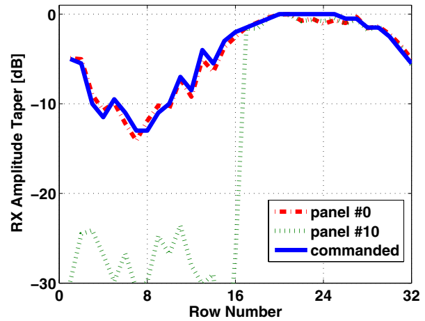
Fig. 4. Commanded and measured beam taper on panel 0 and panel 10 of TerraSAR-X antenna. The first 16 TRMs of panel 10 were switched off.
