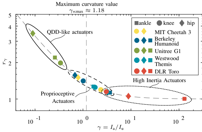
Fig. 6. Inertia-Ratio contribution to impact robustness r_\gamma over Motor-Link Inertia Ratio \gamma in a log-log plot with values of different legged-locomotion systems listed in Tab. II.
