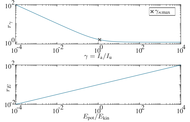
Fig. 3. Factors of the impact robustness r ; energy-ratio term r_E and inertia-ratio term r_\gamma on a log-log plot with base \beta = 10 . With respect to Motor-Link inertia ratio \gamma , the maximum-curvature point \gamma_{\kappa\text{max}} indicates a soft transition between two regions of influence.
