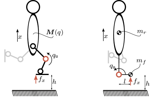
Fig. 4. Vertical drop-height configuration. Left: general case in which dropping a robot from height h with mass matrix M(q) creates a collision force f_x that is mapped to the joints via a Jacobian J_x^T . Right: simplified case in which the mass of the foot is concentrated at the collision point and the collision force is mapped via l to the joint q_u .
