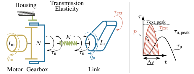
Fig. 1. Schematic diagram of the actuator model. The link inertia is connected to an ideal gearbox and rotor via a transmission elasticity K . An impulse p with sinusoidal torque profile on the external torque \tau_{\text{ext}} and contact time \Delta t excites an oscillation of the gearbox interface torque \tau_u defined at the gearbox output.
