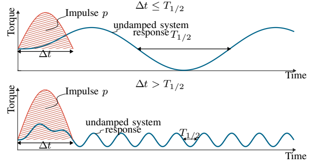
Fig. 2. Not-to-scale illustration of (5) for both short contact times \Delta t \leq T_{1/2} and long contact times \Delta t > T_{1/2} . In both cases the impact excites a torque oscillation. For short contact times, only the first half period is disturbed, while for long contact times the system roughly follows the impact torque profile during the contact.
