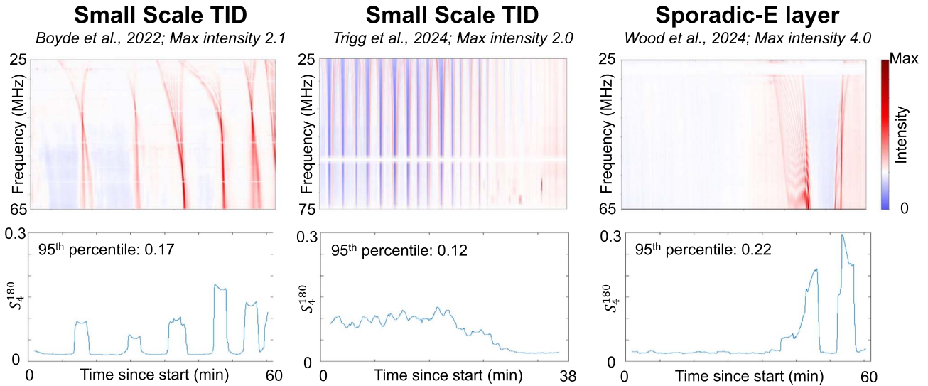
Figure 1. The dynamic spectrum (top row) showing the relative signal intensity as a function of time and of frequency for observations of astronomical radio sources of SSTIDs (Boyde et al., 2022; Trigg et al., 2024) and variations within a sporadic-E layer (Wood et al., 2024). These data have been reprocessed to match the methodology used in the present study. The intensity scales differ between the panels to improve the clarity of this figure. In each case, the minimum value of the intensity scale is zero, and the maximum value is given in the panel heading. The left and right panels both have a duration of one hour; however, the middle panel has a shorter duration of 38 min, as this was the length of the observation. Horizontal white regions correspond to frequency channels removed due to significant radio frequency interference. The lower panels show S_4^{180} as a function of time at a frequency of 44.3 MHz, together with the 95th percentile of this time series.
