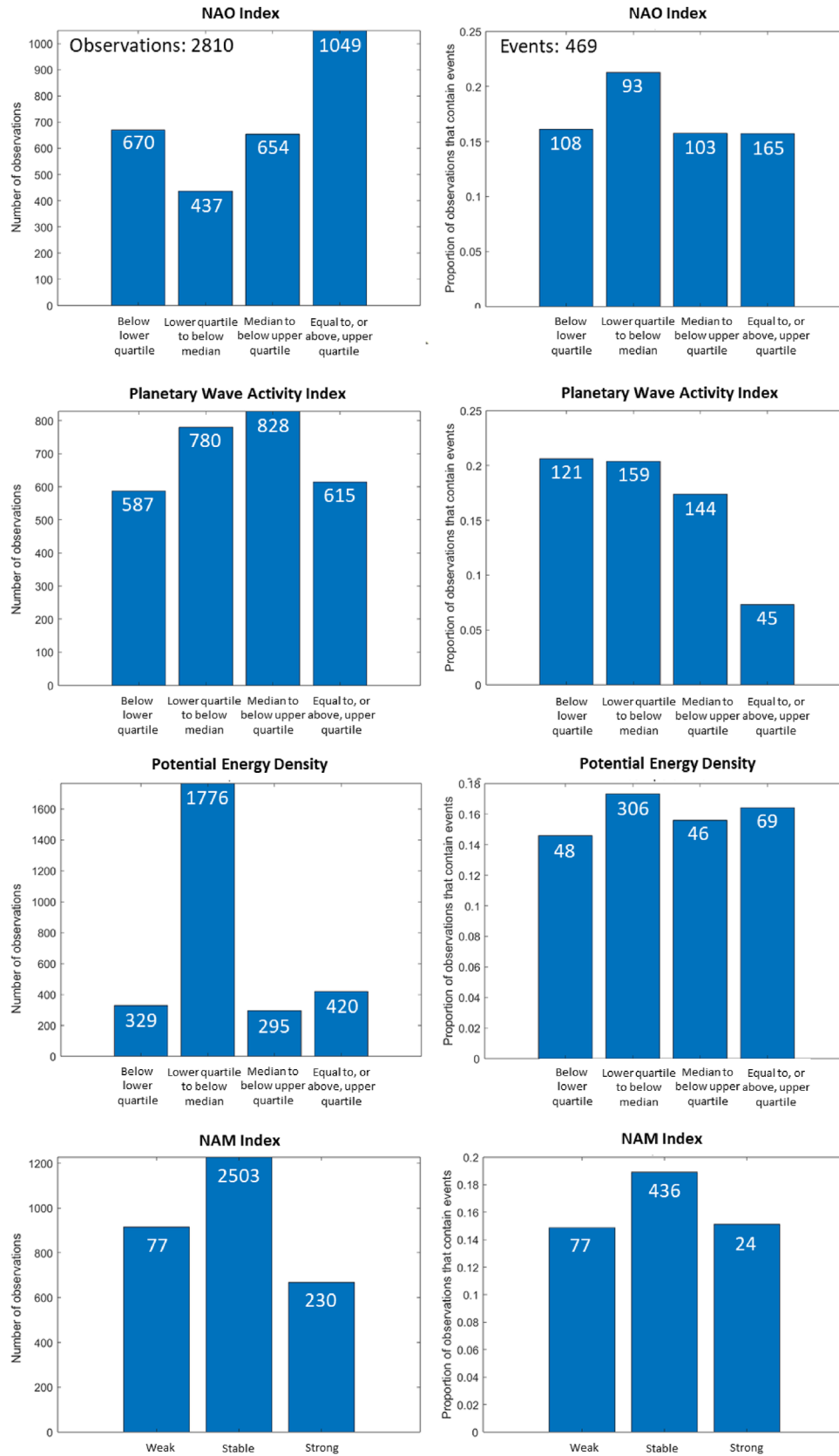
Figure 4. As Figure 2, but for the NAO index (top row), the planetary wave activity index (second row), the potential energy density of AGWs (third row), and the NAM index (lower row). The planetary wave activity index and the potential energy density of the AGWs were observed at the Environmental Research Station (UFS) at Schneefenerhaus, Germany (47.04° N; 10.98° E).
