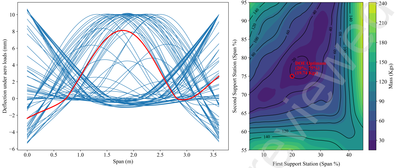
Figure 10: Mass and deflection trends of Flaperon-3 for varying support station locations
