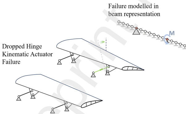
Figure 7: Dropped-Hinge kinematic failure case and corresponding simplified structural model (see also (14))
