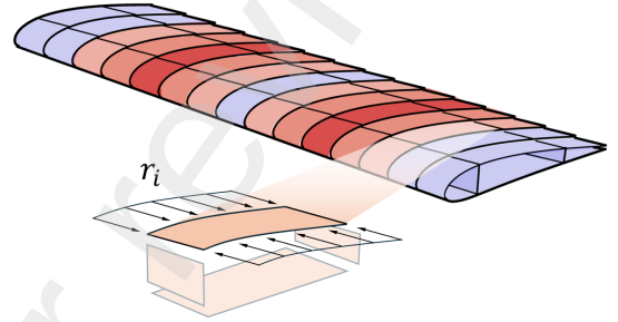
Figure 9: Membrane and shear flows r_i recovered from PreDoCS and used to panel sizing in lightworks
