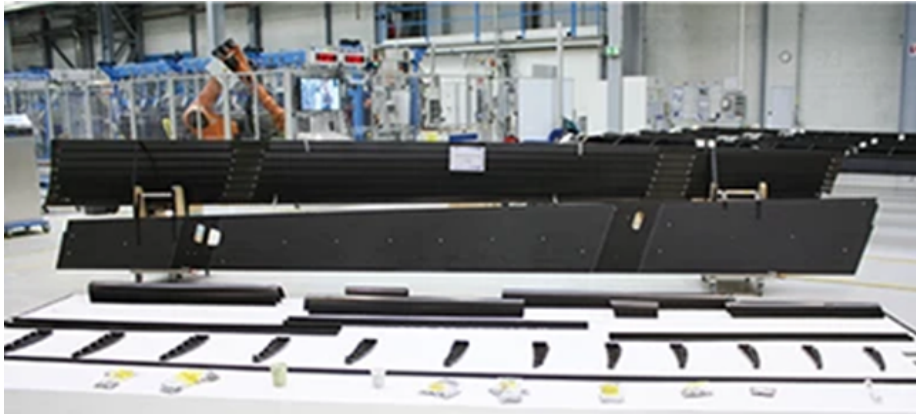
(a) Today's differential concept for an A321 composite flap (4) and corresponding design concept (5)
