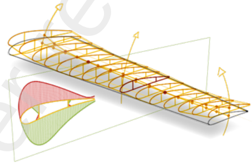
Figure 8: Beam idealisation of the flap-eron and recovery of sectional and panel loads using PreDoCS
