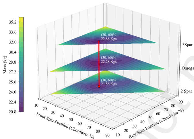
Figure 15: Mass sensitivity of Flaperon-1 to reinforcement layouts, with lightest configuration of each concept traced in red
