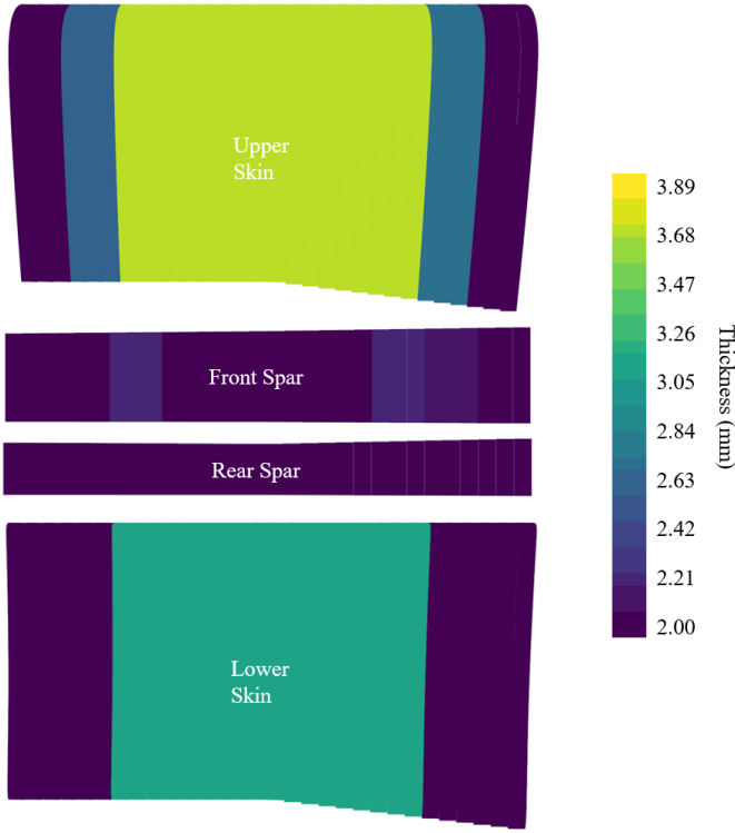
Figure 16: Minimum-mass configuration of Flaperon-1: supports at (20%, 75%) span, and two spars at (30%, 60%) chord
