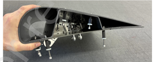
(b) High-TRL modular composite flap concepts: Composite Multi-Spar Flap (CMF, 2015) ©Radius Engineering (6), Advanced Multi-Cell Flap (AMF, 2021) ©FACC (7), and DLR's omega-backbone concept for the F25 outboard flaperon-3 (from left to right)
