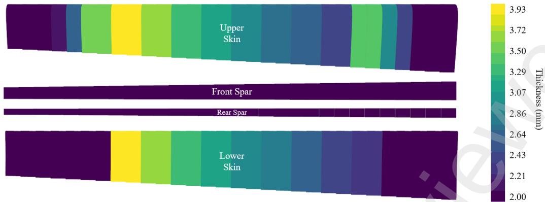
Figure 12: Minimum-mass configuration of Flaperon-3: supports at (20%, 75%) span, and two spars at (30%, 65%) chord
