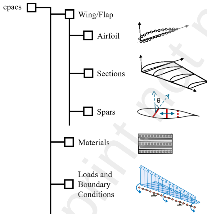
Figure 4: Data structure and contents of a CPACS file
