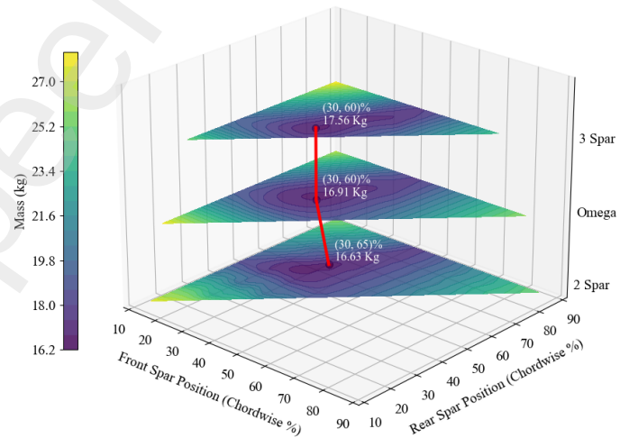
Figure 11: Mass sensitivity of Flaperon-3 to reinforcement layouts, with lightest configuration of each concept traced in red
