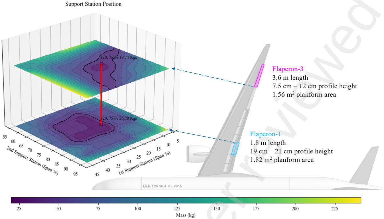
Figure 17: Difference in optimum configurations of Flaperons 1 and 3 of the DLR-F25
