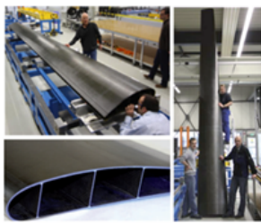
(b) High-TRL modular composite flap concepts: Composite Multi-Spar Flap (CMF, 2015) ©Radius Engineering (6), Advanced Multi-Cell Flap (AMF, 2021) ©FACC (7), and DLR's omega-backbone concept for the F25 outboard flaperon-3 (from left to right)
