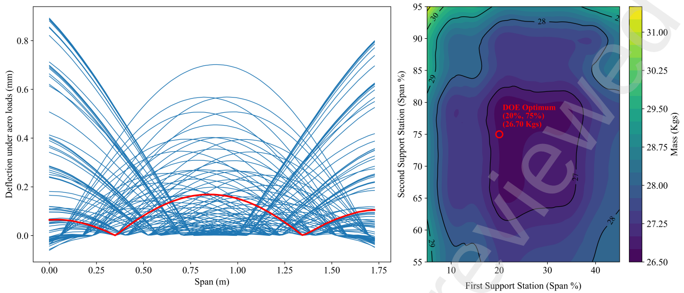
Figure 14: Mass and deflection trends of Flaperon-1 for varying support station locations
