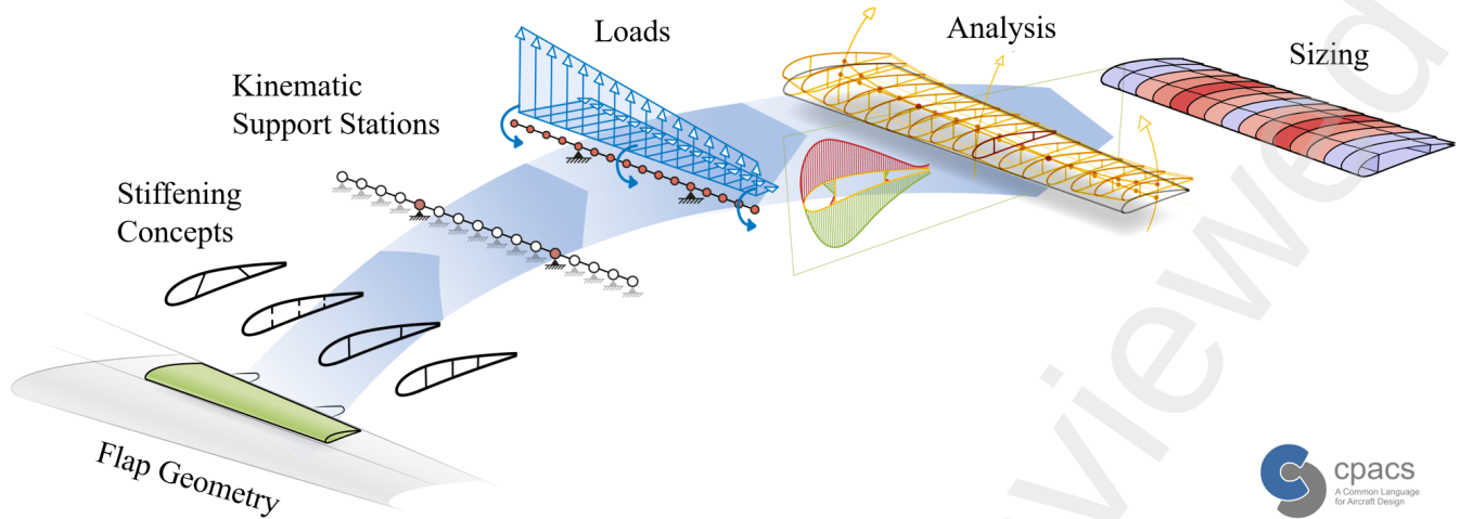
Figure 3: Overview of the preliminary structural design workflow for high-lift devices
