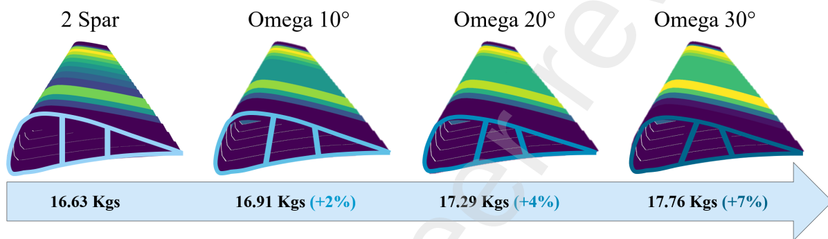
Figure 13: Quantifying mass penalty of Flaperon-3 by rotating spars for ease of production (omega configuration)
